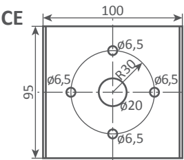
Platine de fixation murale / Wall mounting plate
