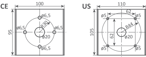
Platine de fixation murale / Wall mounting plate
