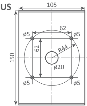
Platine de fixation murale / Wall mounting plate
