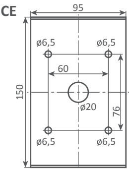
Platine de fixation murale / Wall mounting plate
